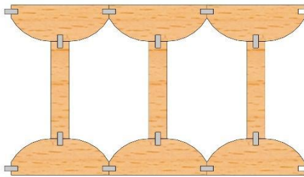
FIGURE. Schematic drawing of a hollow-core wall & intermediate-floor element.
