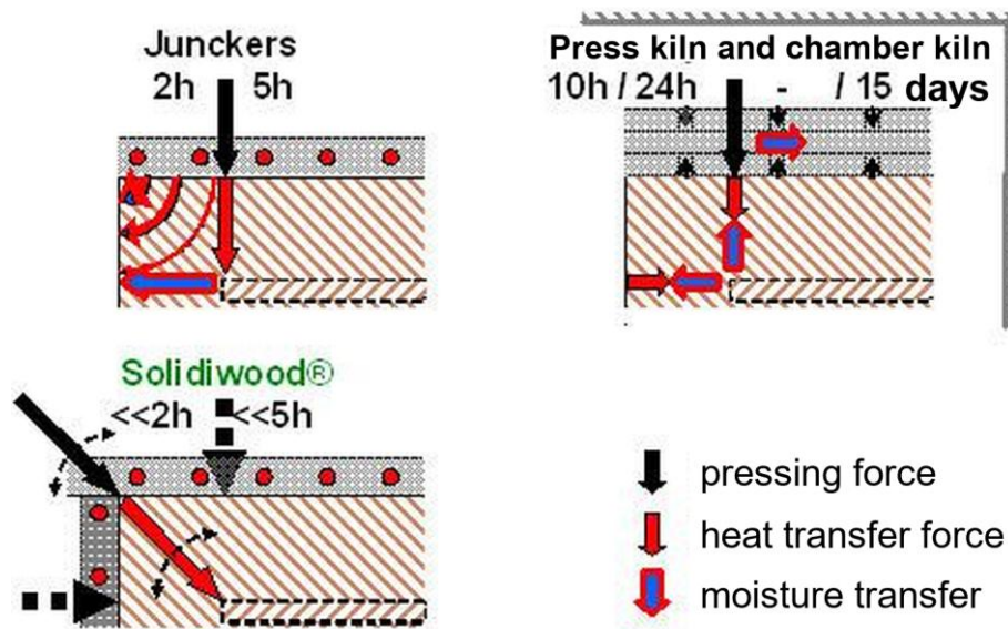
FIGURE. Junckers and Solidiwood® vs. press kiln and chamber kiln
